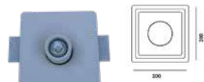
Fitting-Ceiling Metal-1XGU10
